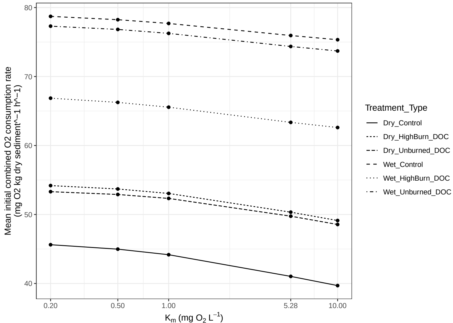
Sensitivity of total modeled O 2 consumption to K m
