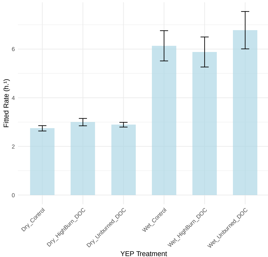
Abiotic Rates (kL)
