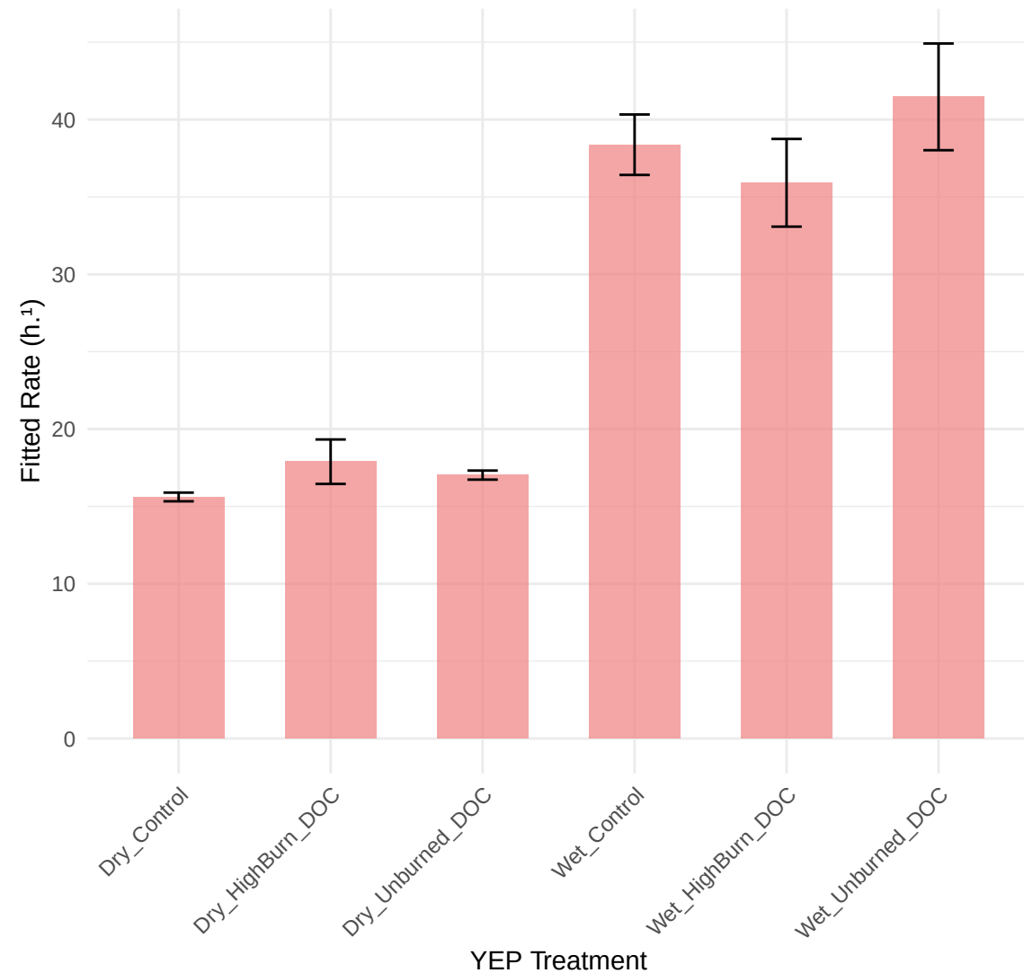
Biotic Rates (Vmax)
