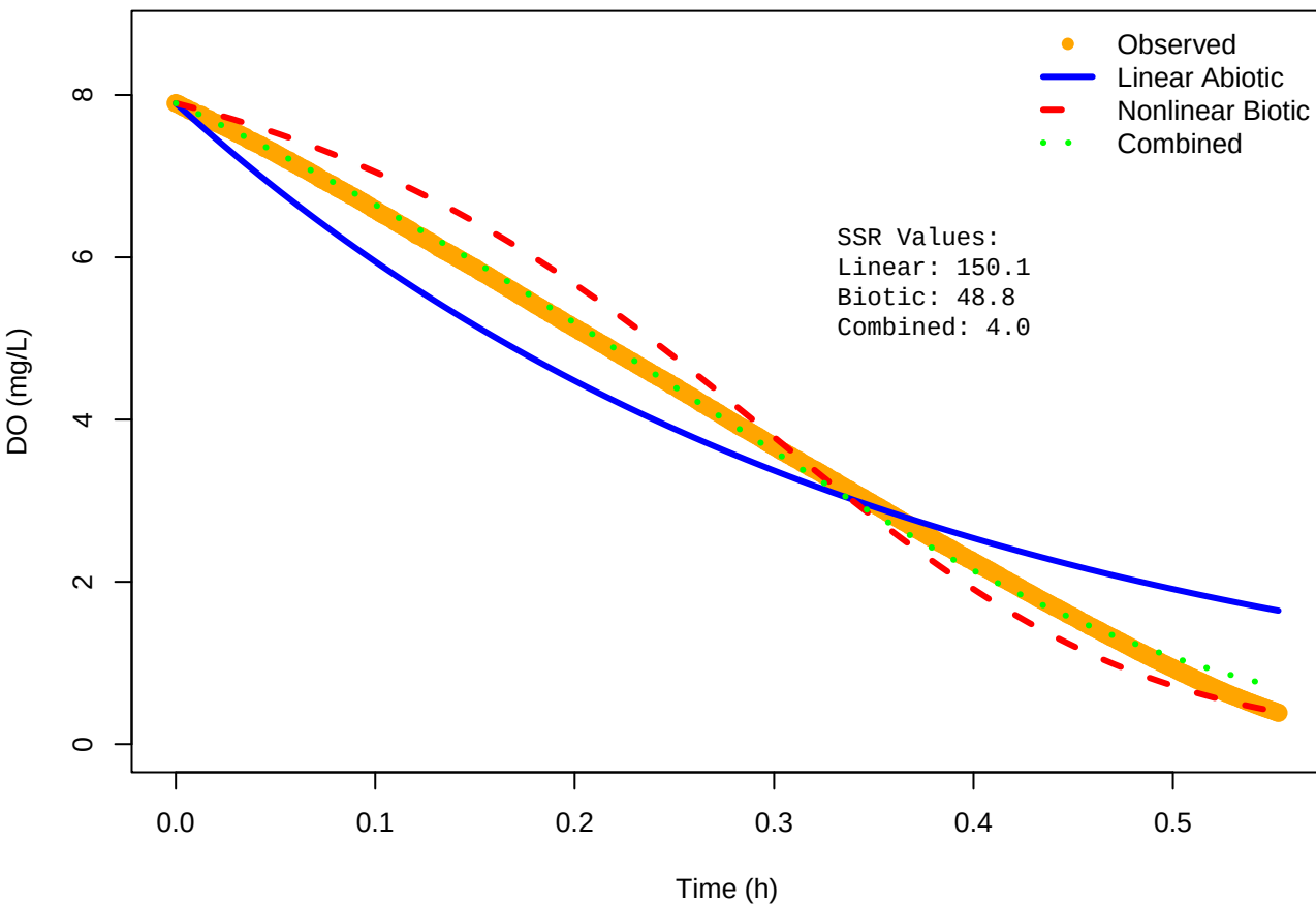
Nonlinear Biotic SSR = 48.8
