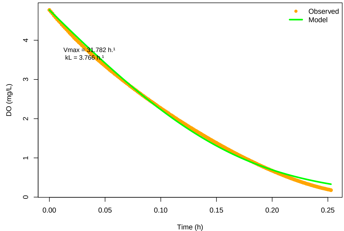
Combined SSR = 0.9
