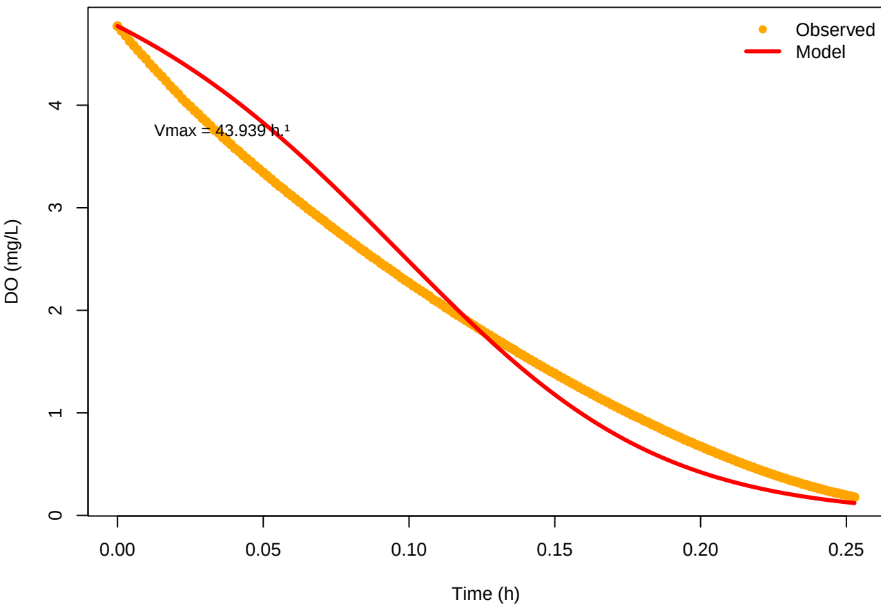
Nonlinear Biotic SSR = 14.3
