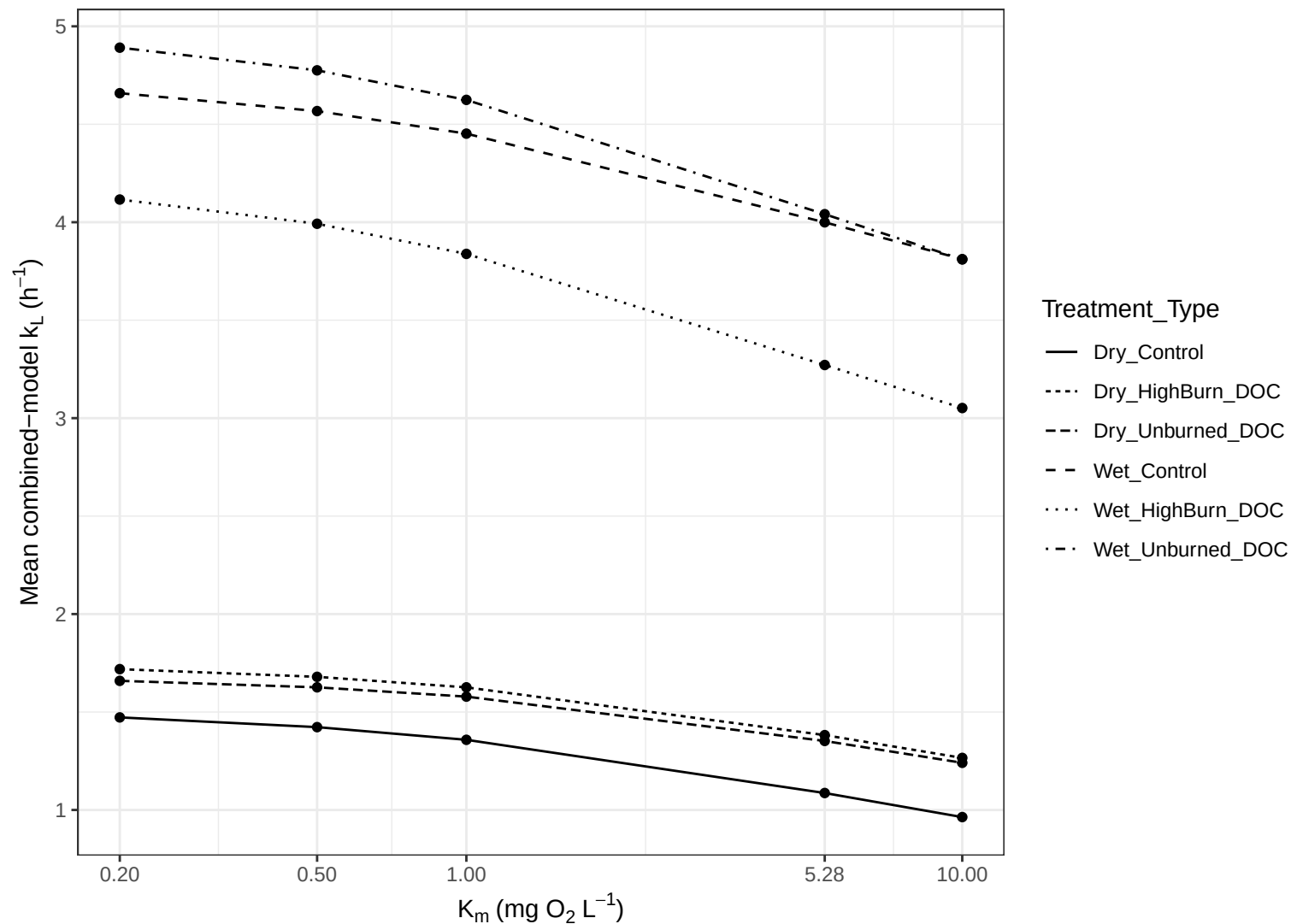
Sensitivity of fitted k_L to fixed K_m
