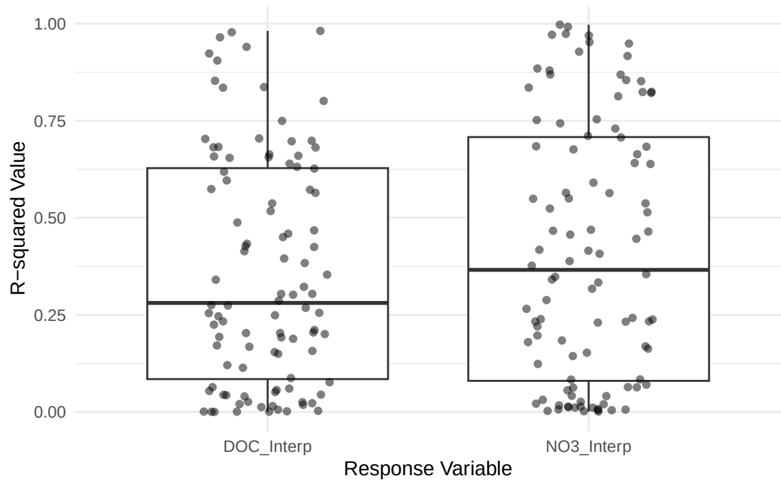
Distribution of R-squared Values Across Iterations
