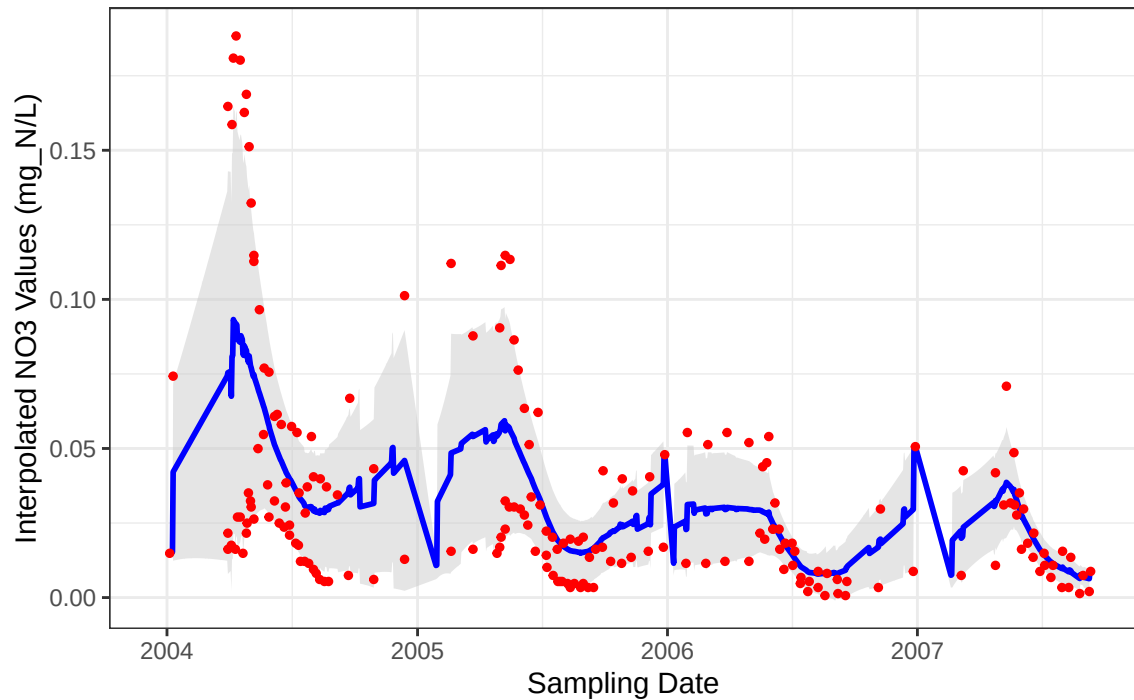
Time Series of NO 3 Interpolated Values with Distribution Ribbon
