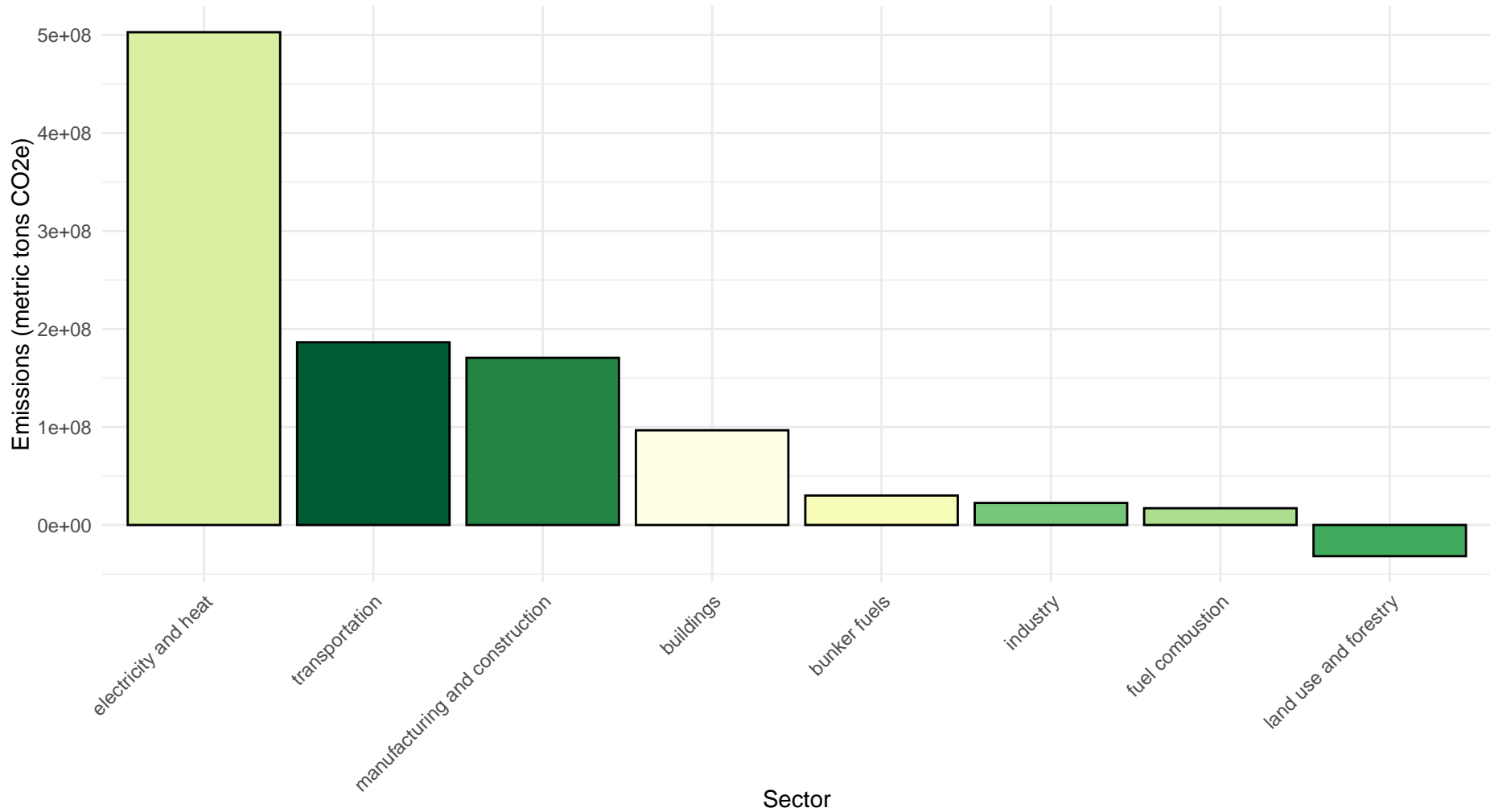
Japan Greenhouse Gas Emissions by Sector (2022)
