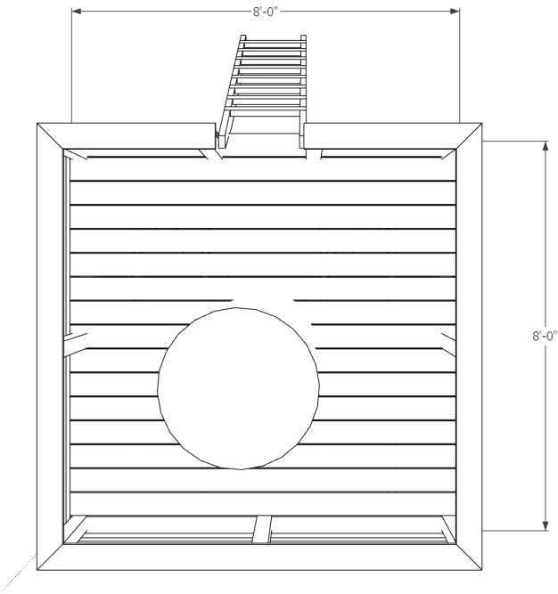
Fig. 1.1 - Tree Fort Plan
