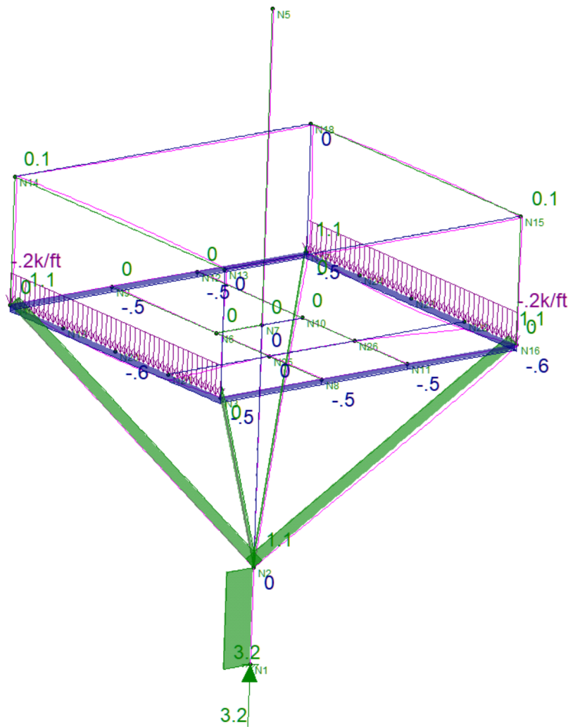
Fig. 2.1 - Strut Axial Forces
