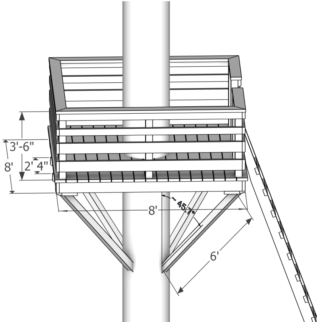
Fig. 1 - Tree Fort Dimensions
