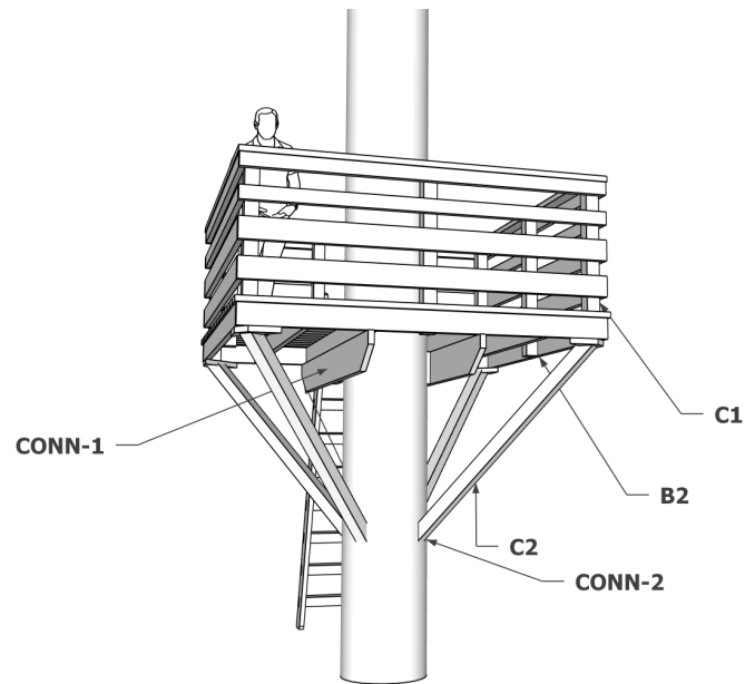
Fig. 2 - Component Labels
