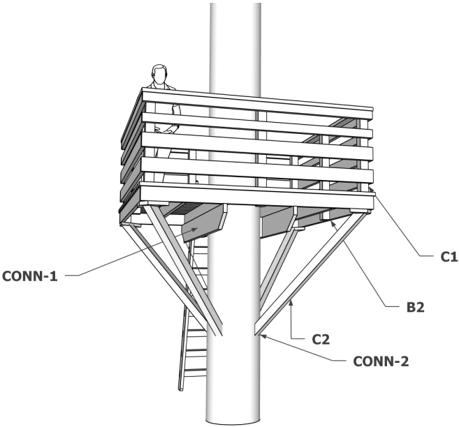
Fig. 2 - Component Labels
