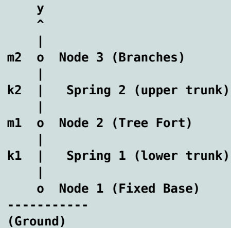
AI schematic model of tree + tree-fort system
