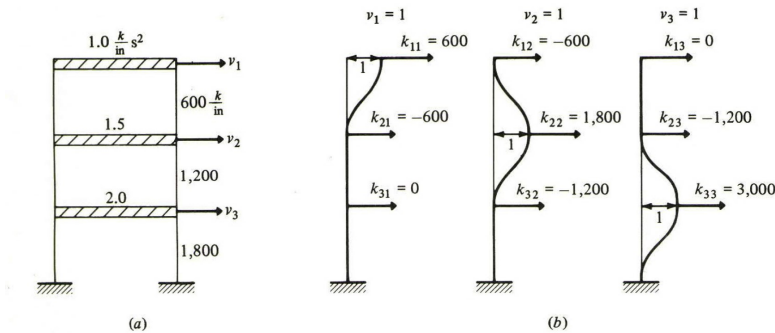
Fig. 1 - Structural Model
