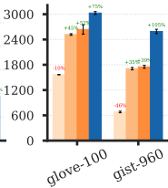
Usearch
