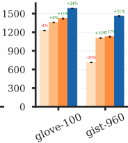
Usearch
