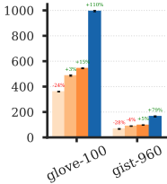
Throughput (QPS)
