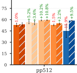
Throughput (tokens/s)
