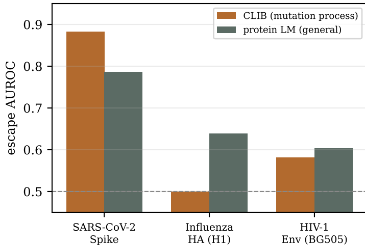
(b) transferable component: process vs protein
