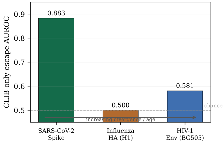
(a) mutation-accessibility prior: viral-age-dependent scope
