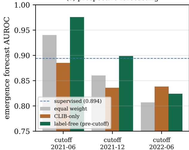
(a) prospective forecasting
