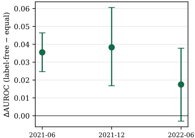
(b) improvement, 95% CI
