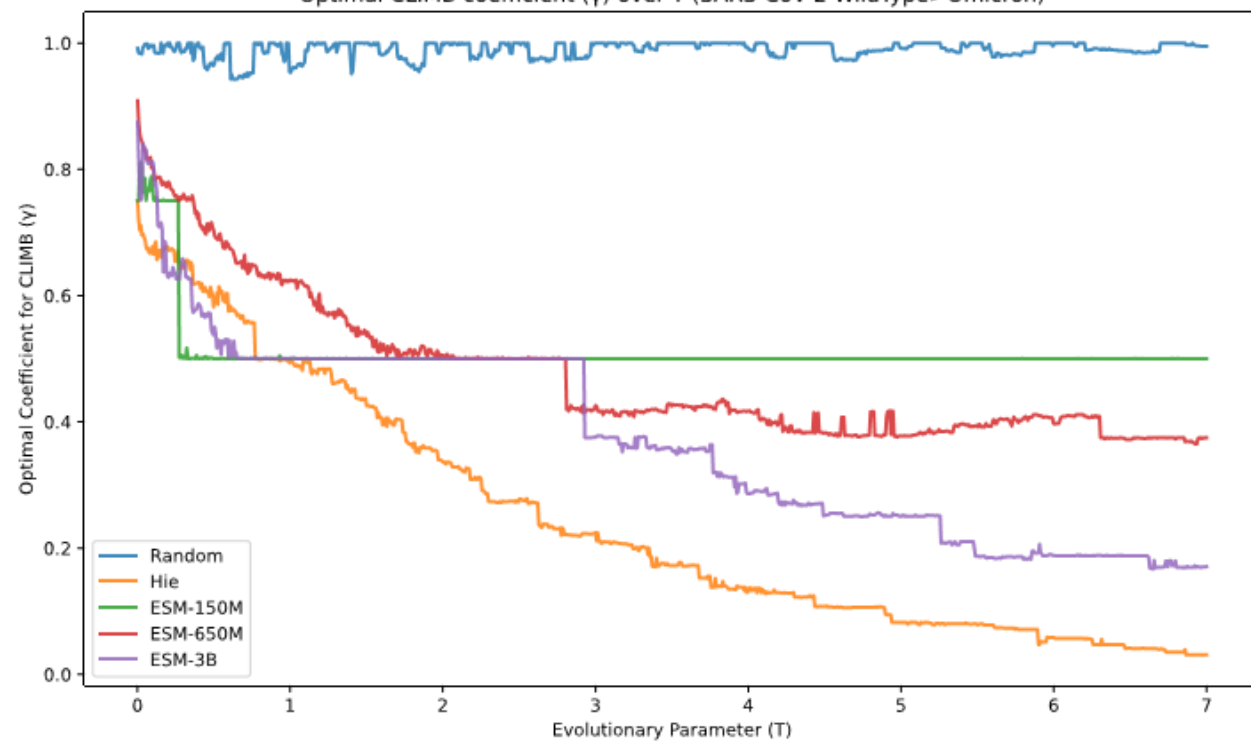
Optimal CLIMB coefficient ( \gamma ) over T (SARS-CoV-2-wildtype>Omicron)
