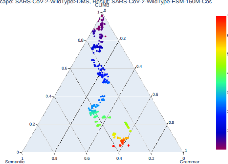
Mean Rank Minimizers for SARS-CoV-2-WildType Escape: SARS-CoV-2-WildType>DMS, Result: SARS-CoV-2-WildType-ESM-150M-Cos
