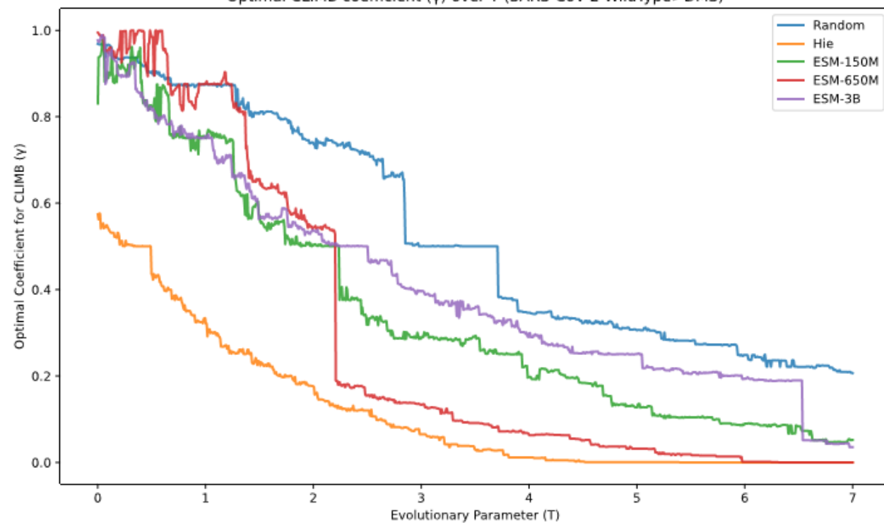
Optimal CLIMB coefficient ( \gamma ) over T (SARS-CoV-2-wildtype>DMS)
