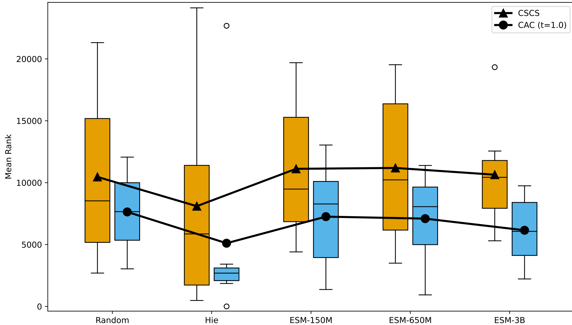
Box-whisker plot of SARS-CoV-2-WildType>Delta for CSCS and CAC (t=1.0)
