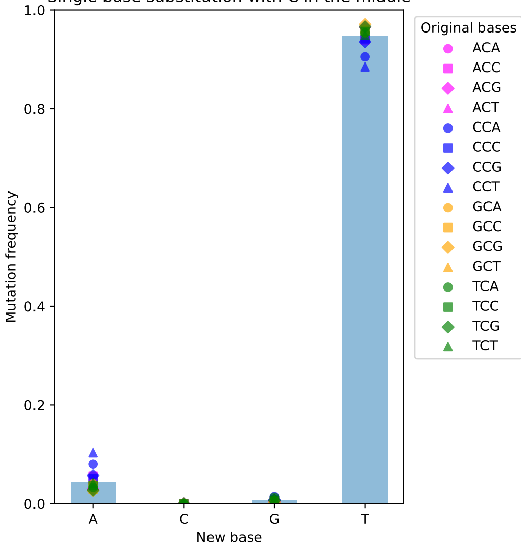
Single base substitution with C in the middle
