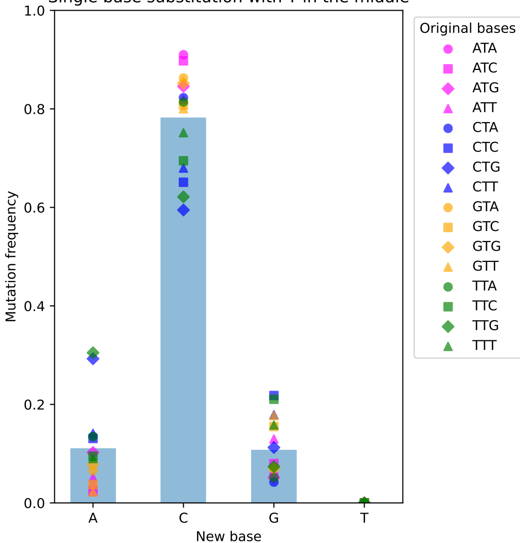
Single base substitution with T in the middle
