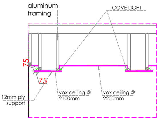
A DETAIL- A
