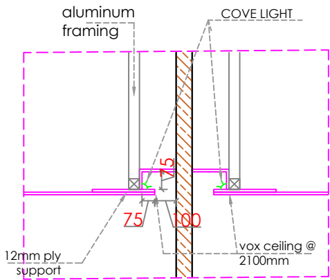
B DETAIL- B
