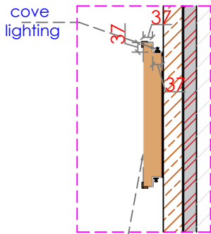
2 DETAIL- 2
