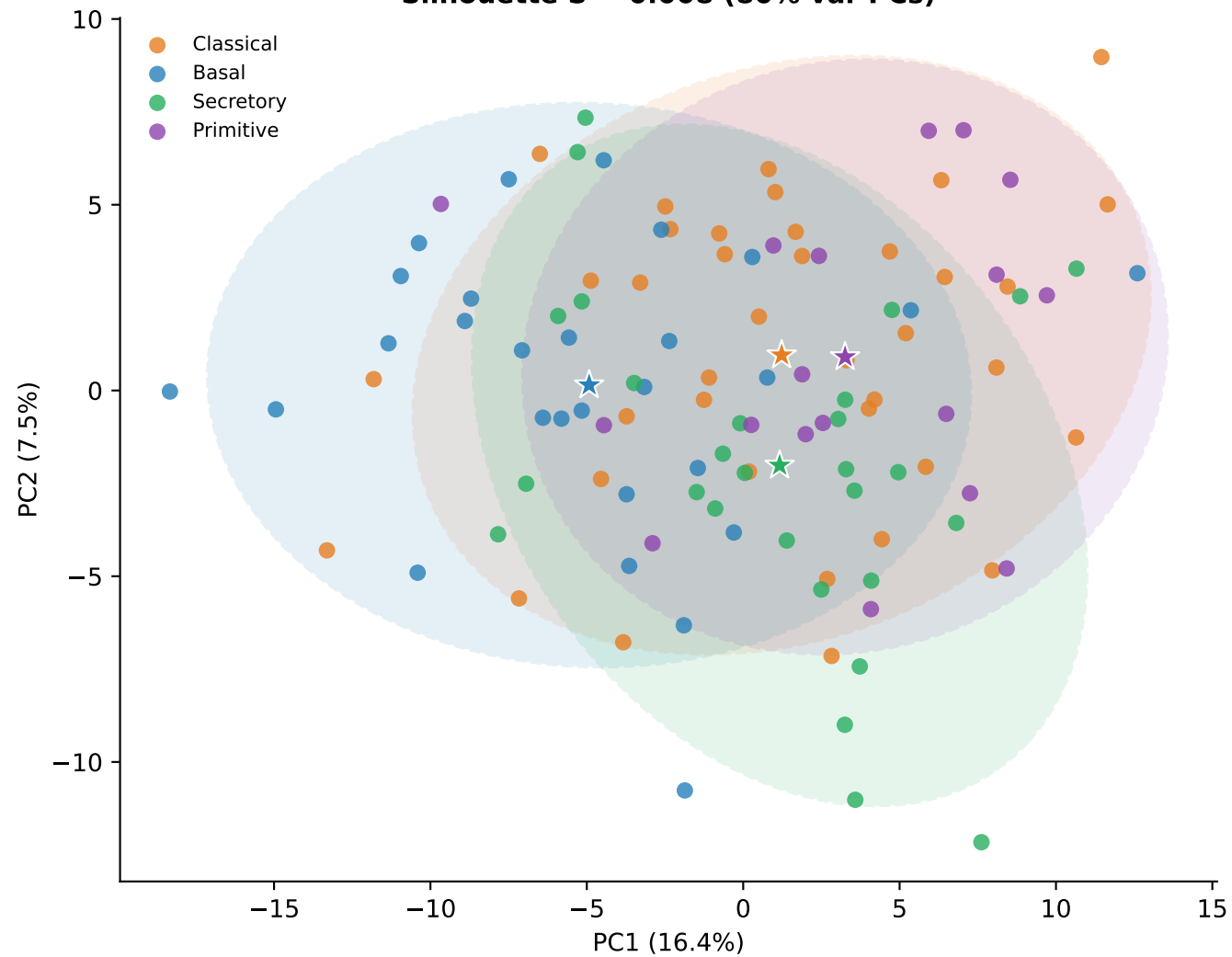
RPPA Silhouette S = 0.008 (80% var PCs)
