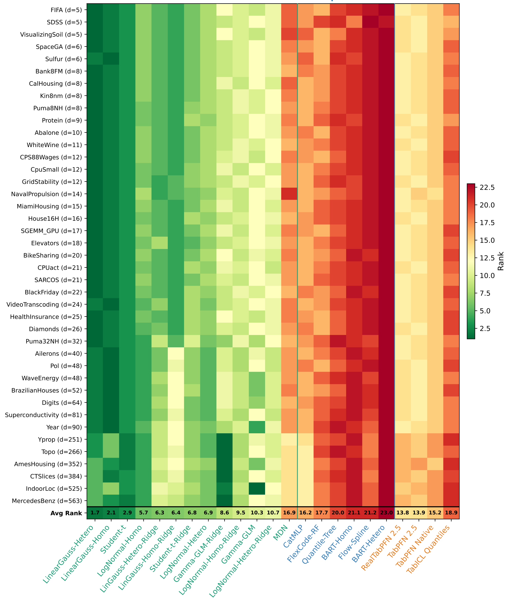
Fit Time — Rankings (n=1000, Real)
