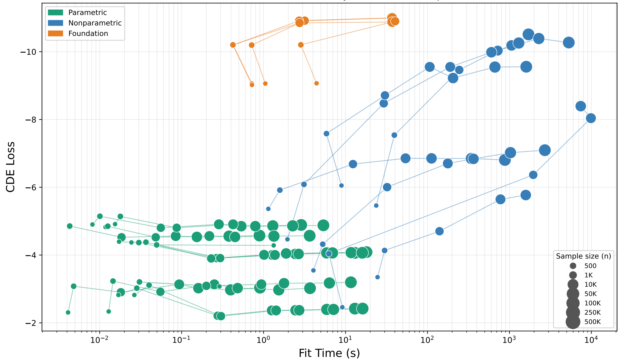
SDSS Scaling: Fit Time vs CDE Loss lower CDE Loss values are better (y-axis inverted: top = better)
