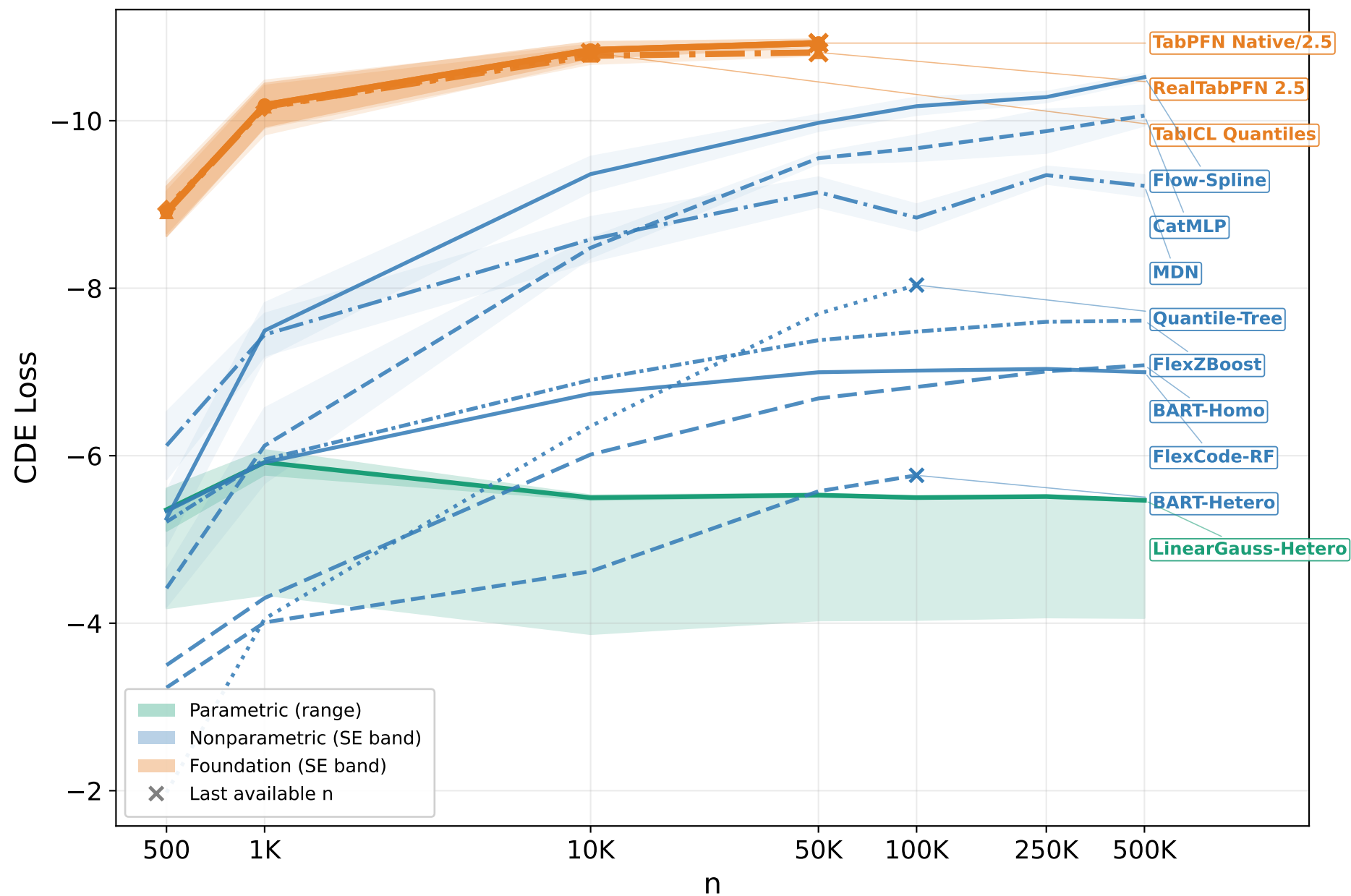
CDE Loss vs Sample Size — SDSS (top is better)
