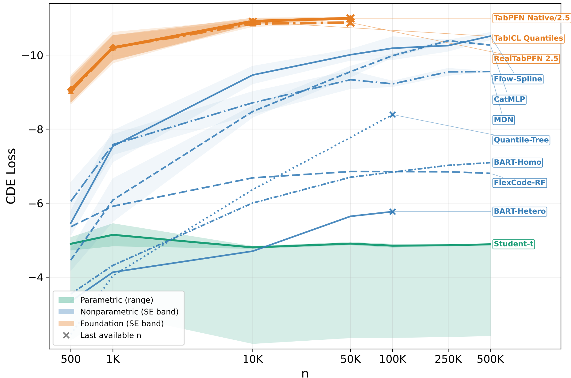
CDE Loss vs Sample Size — SDSS (lower is better, top = better)
