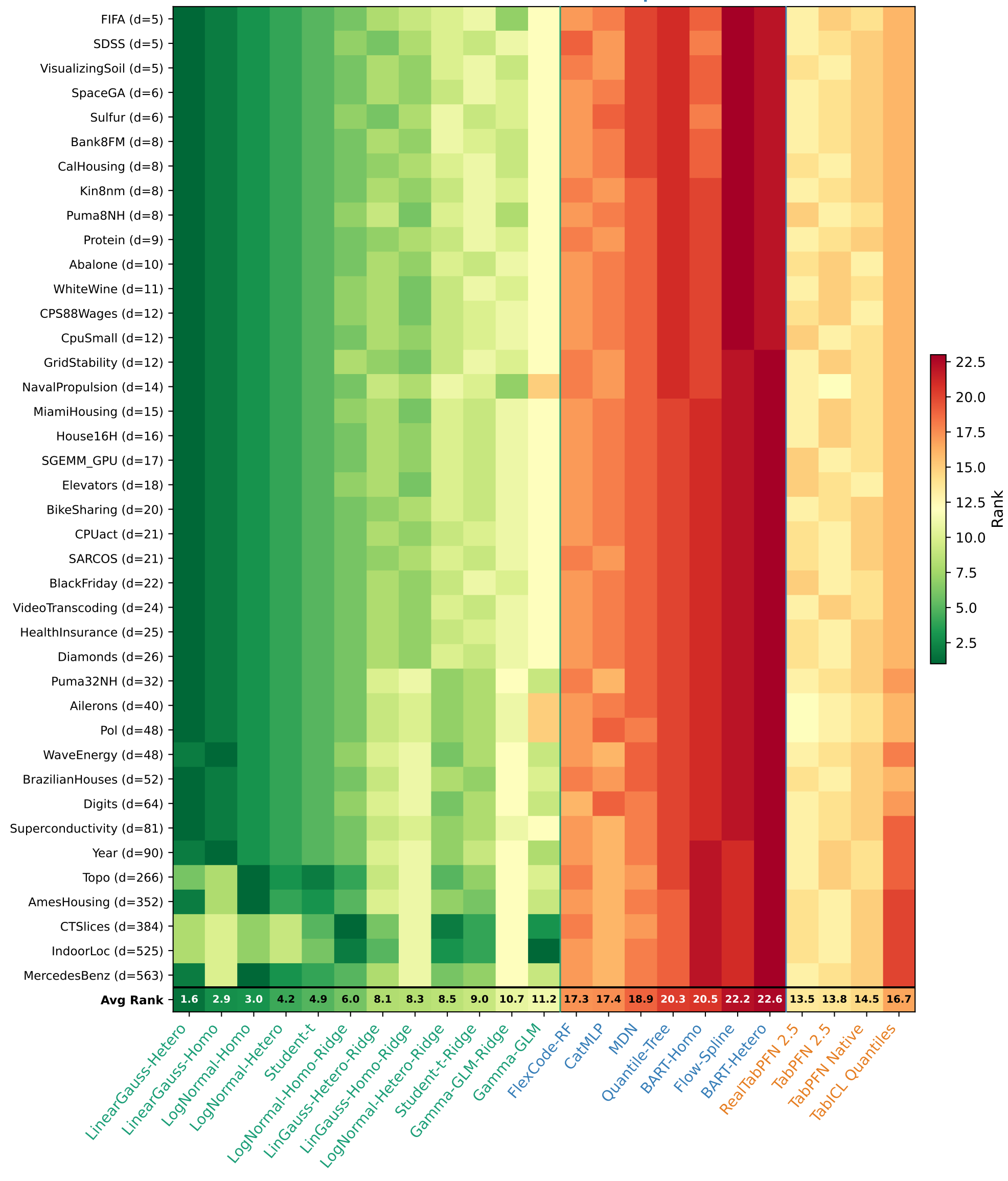
Fit Time — Rankings (n=50, Real)
