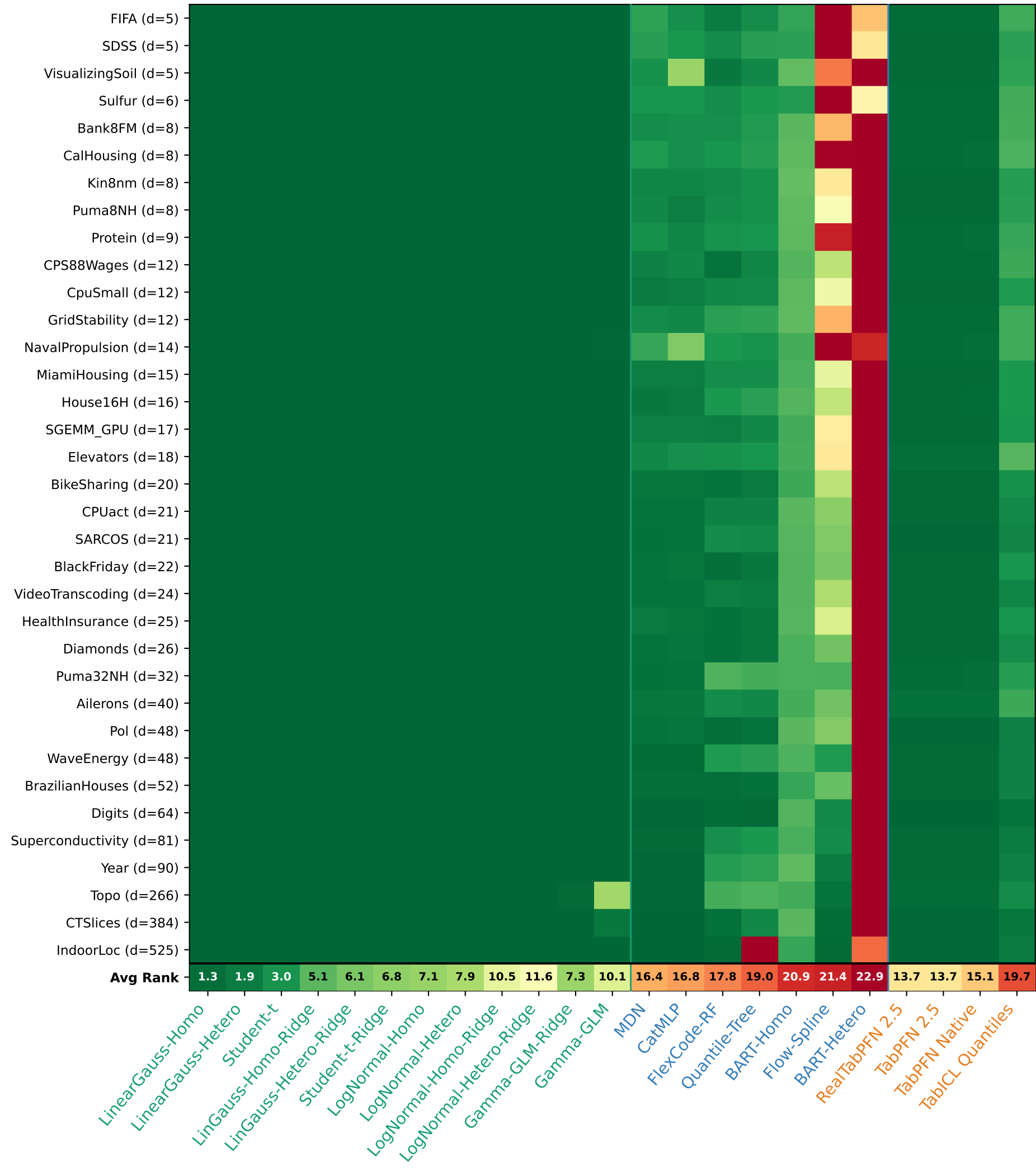
Fit Time — Raw Values (n=5000, Real) Parametric Nonparametric Foundation
