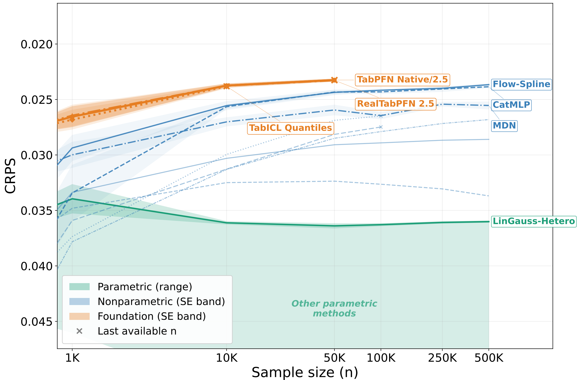
CRPS vs Sample Size — SDSS (top = better)
