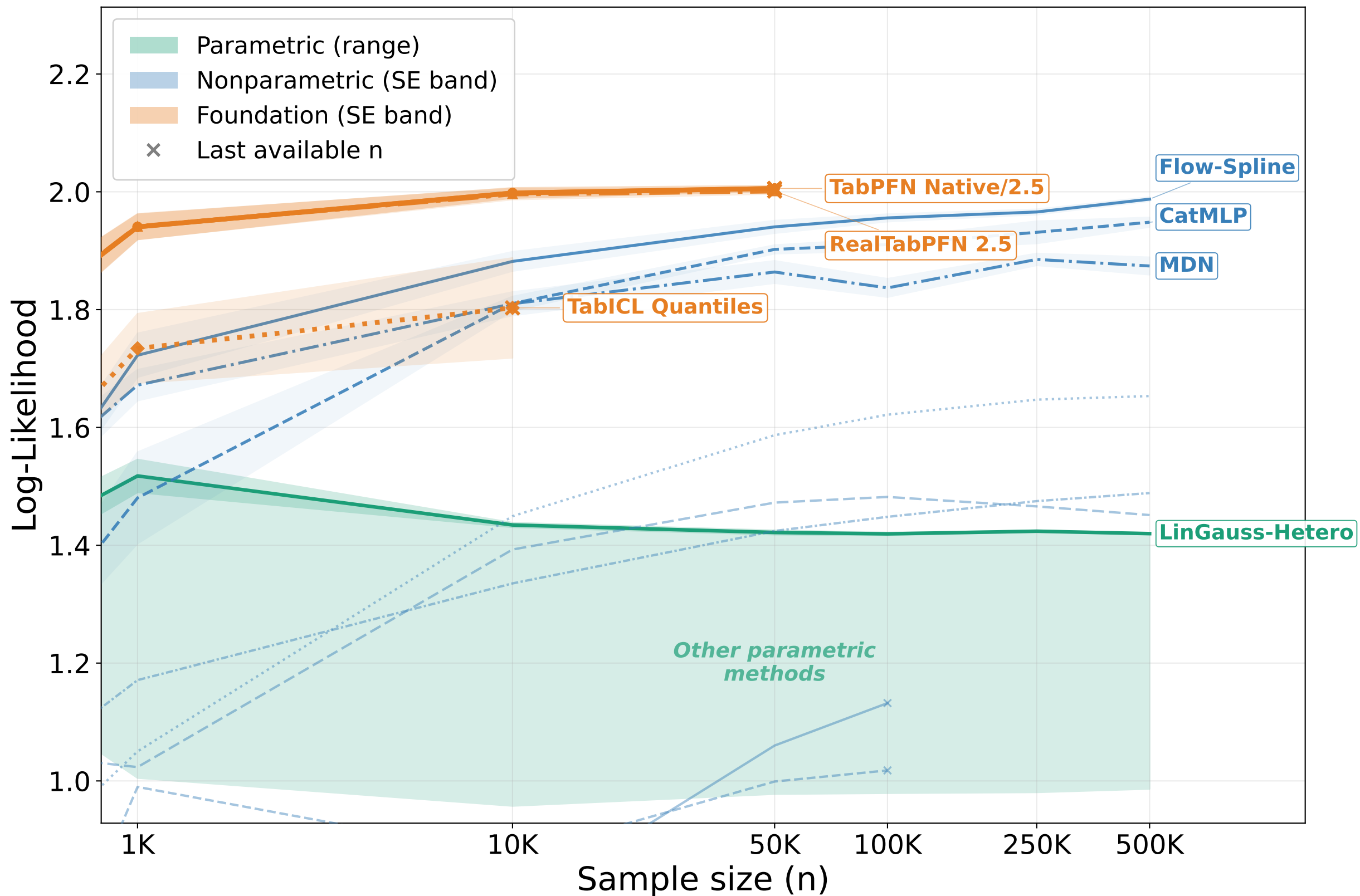
Log-Likelihood vs Sample Size — SDSS (top = better)
