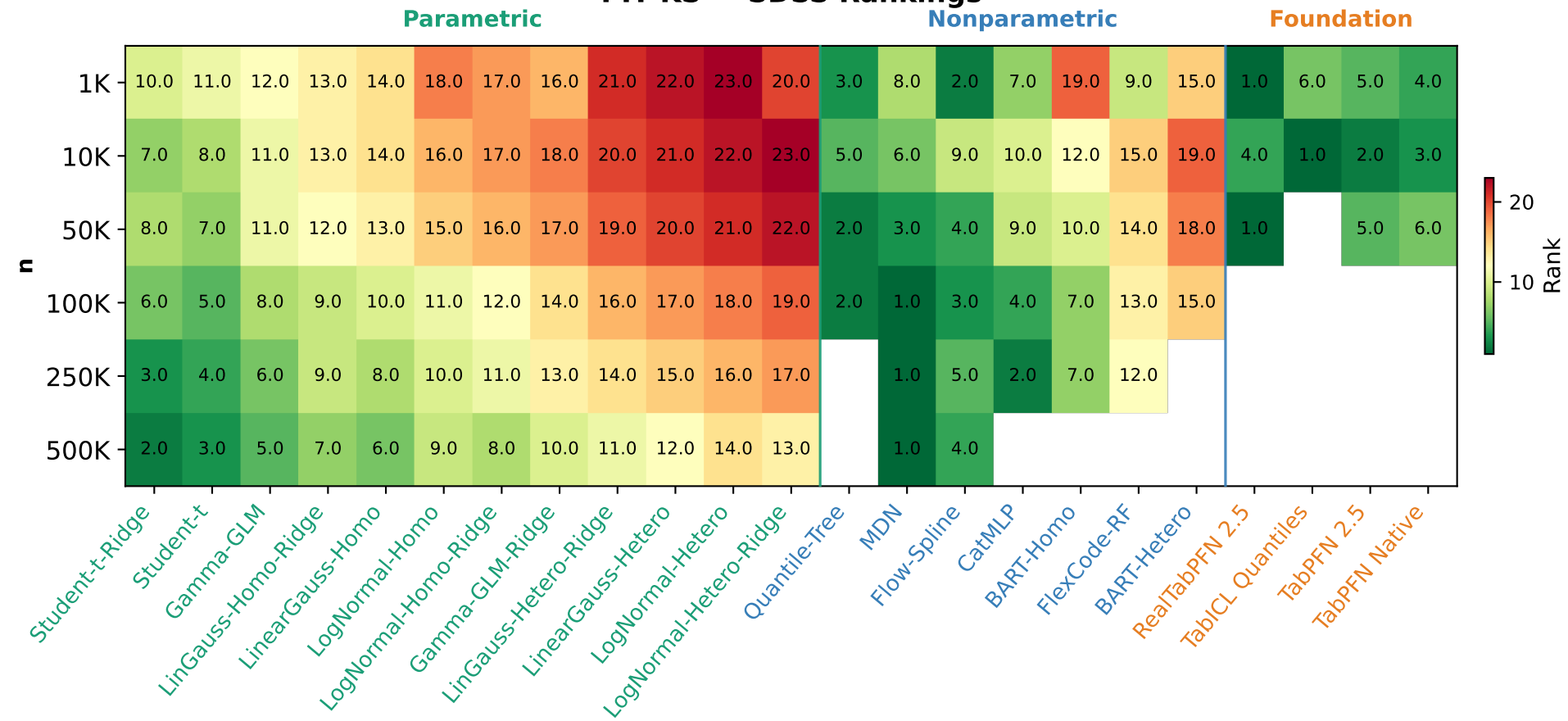
PIT KS — SDSS Rankings
