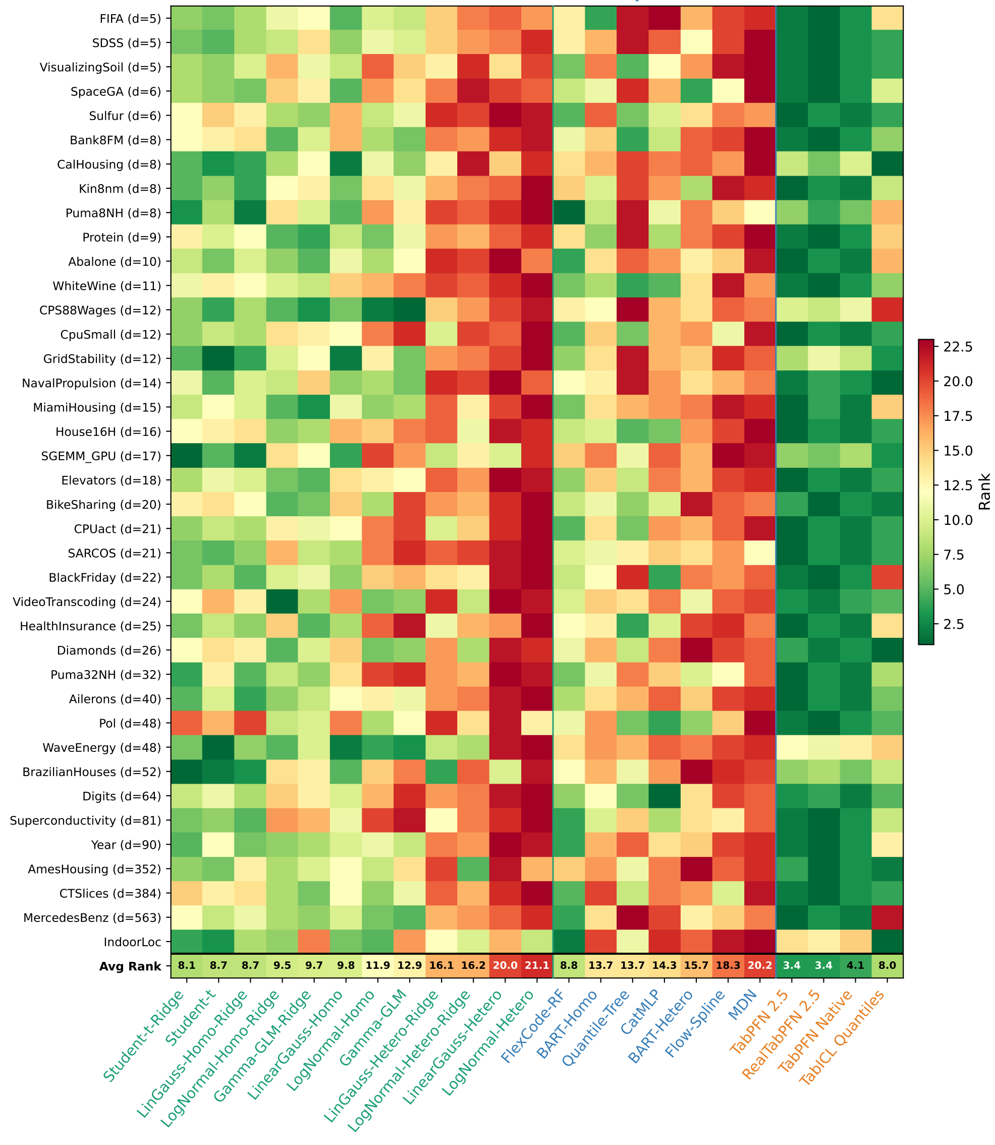
CDE Loss — Rankings (n=50, Real)
