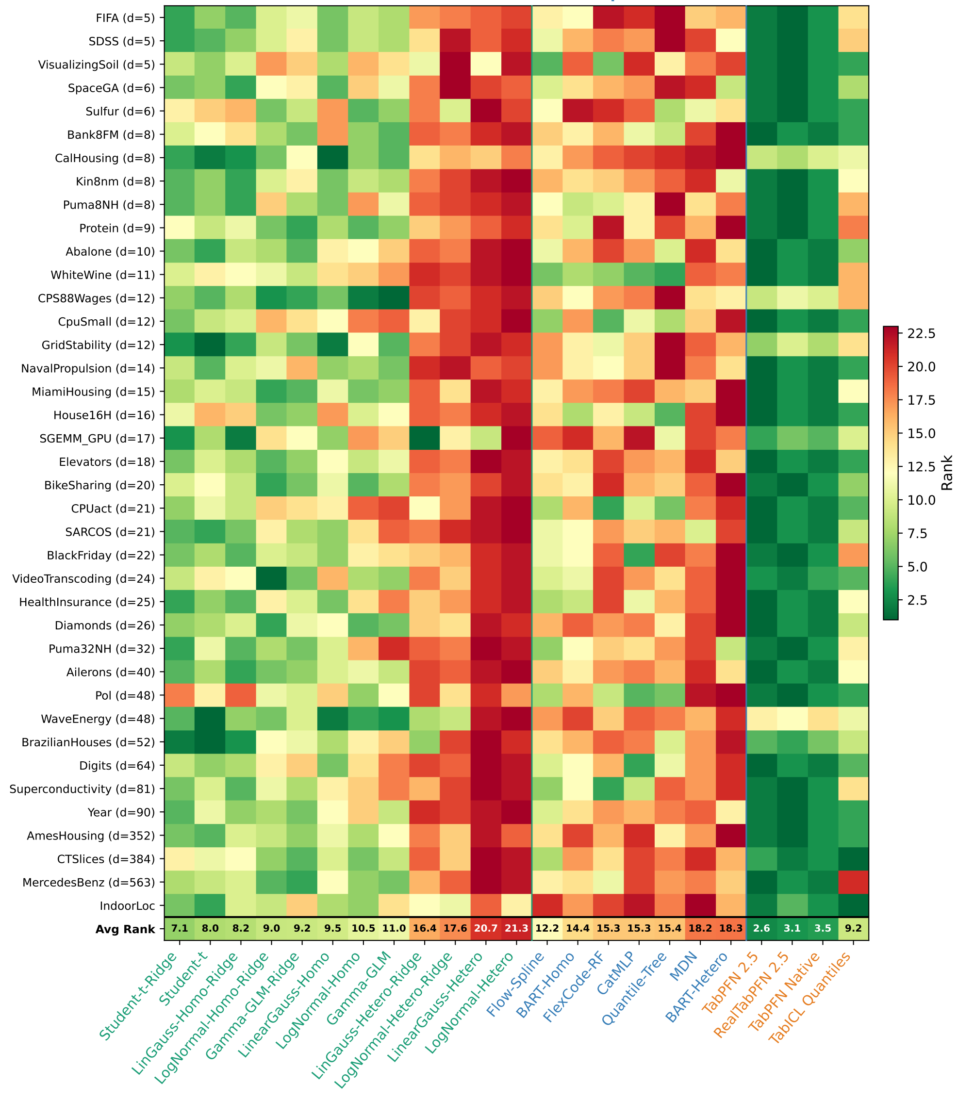
Log-Lik — Rankings (n=50, Real)
