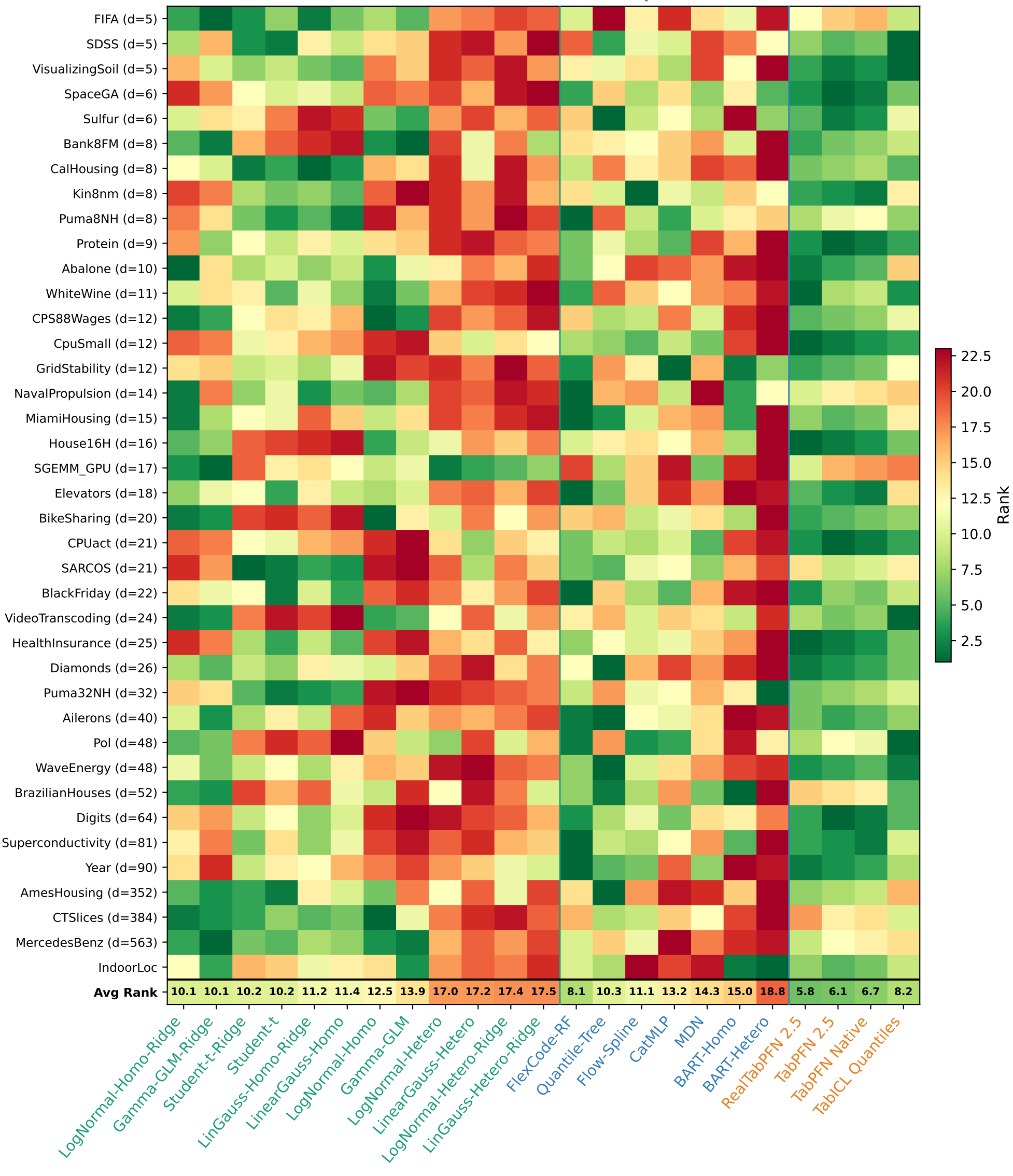
PIT KS — Rankings (n=50, Real)
