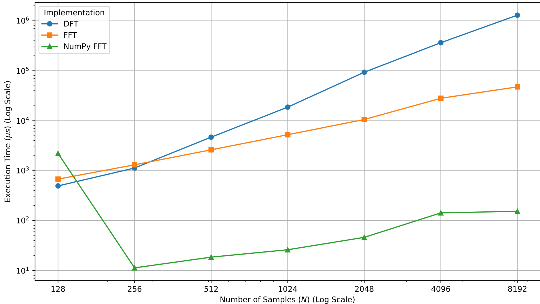
Fourier Transform Performance Benchmark
