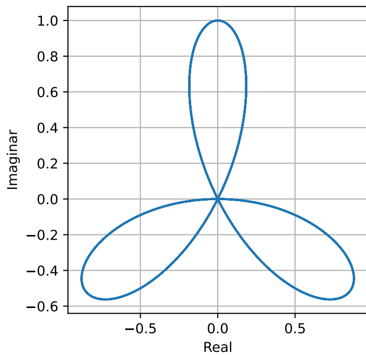
\omega=7
