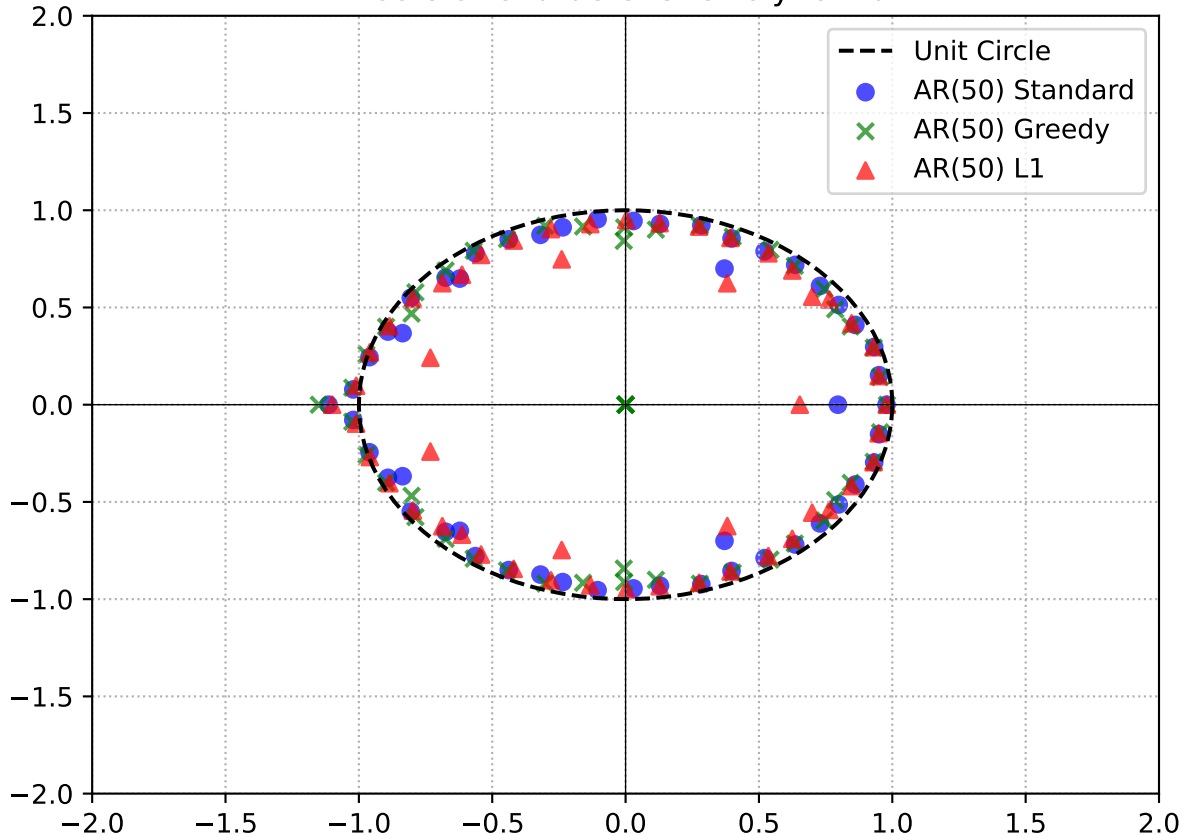
Roots of Characteristic Polynomial
