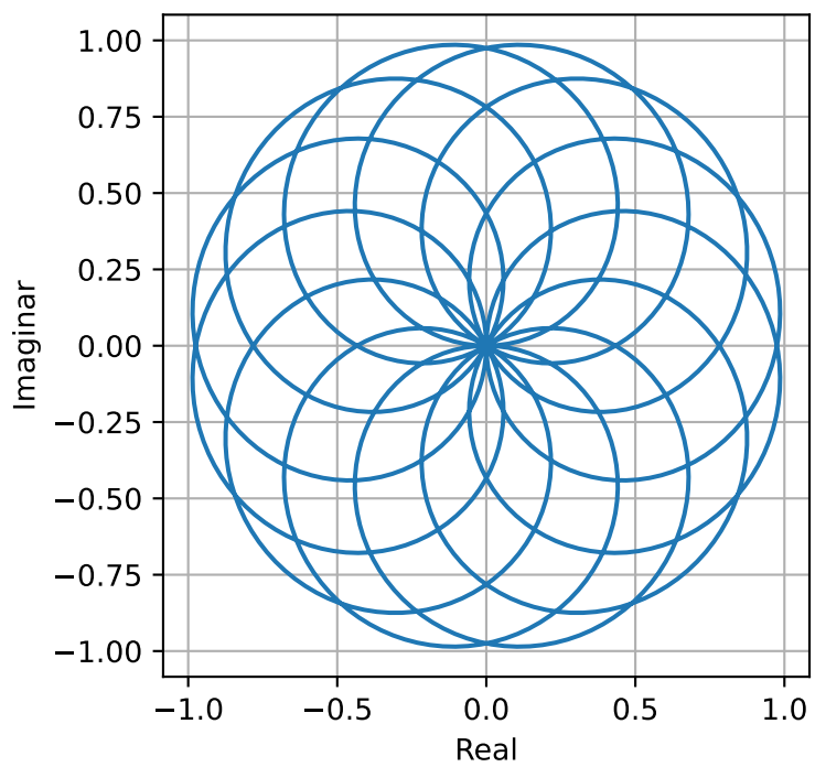
\omega=7
