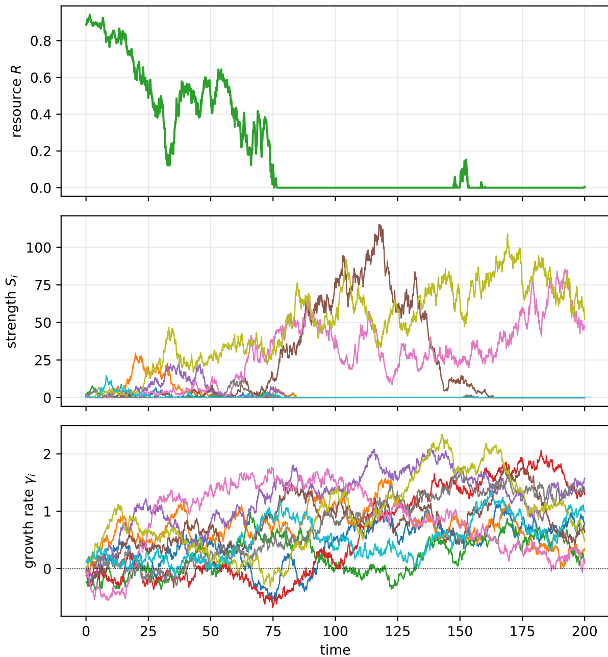
Step 0: pure resource-limited growth ( N = 10 , no wars)
