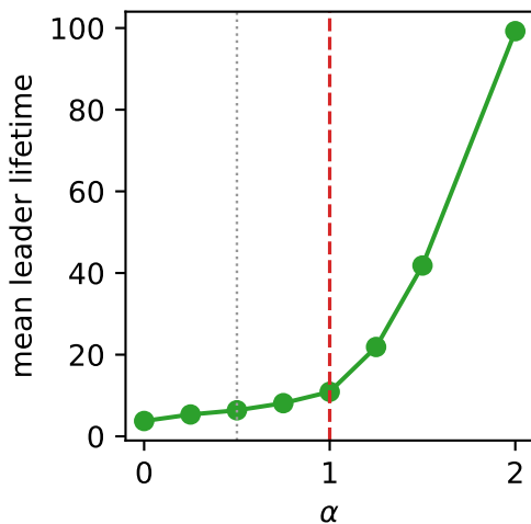
(b) hegemon longevity ( \alpha=1 dashed)
