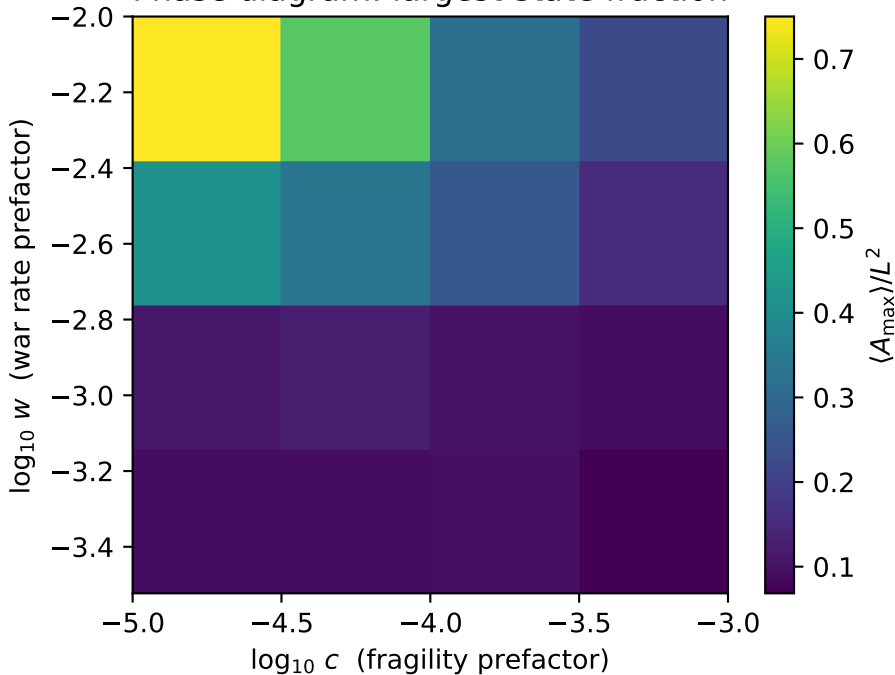
Phase diagram: largest-state fraction
