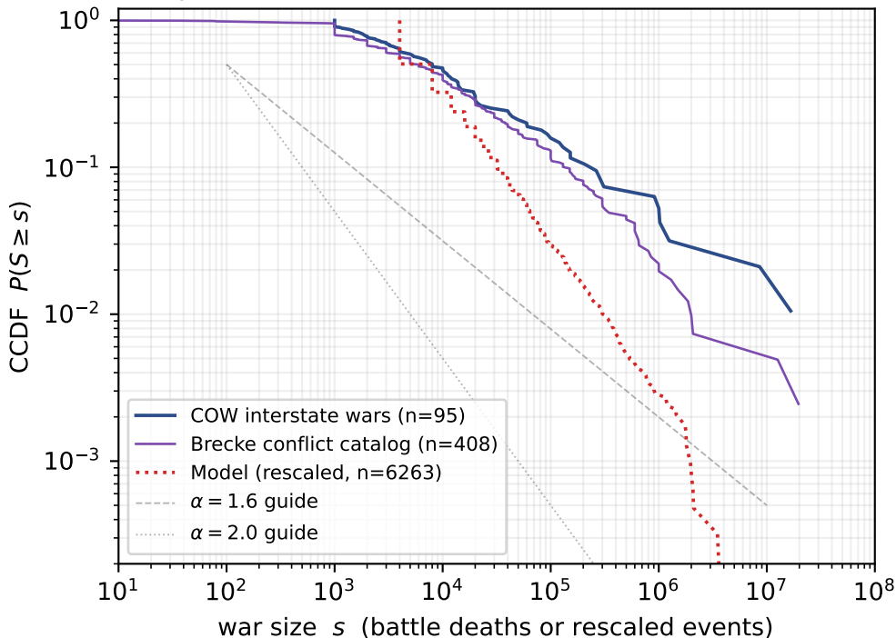
Empirical war-size distributions vs. minimal model
