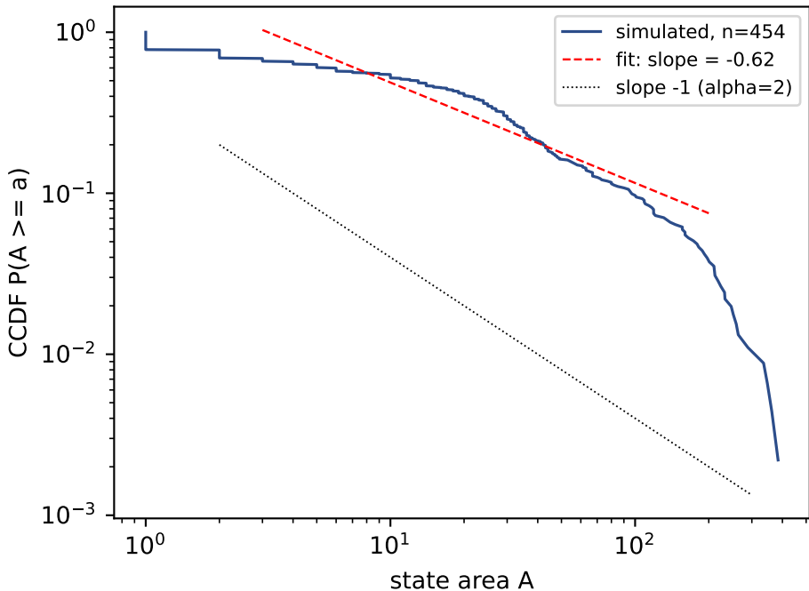
State-size CCDF (snapshots across 3 seeds)
