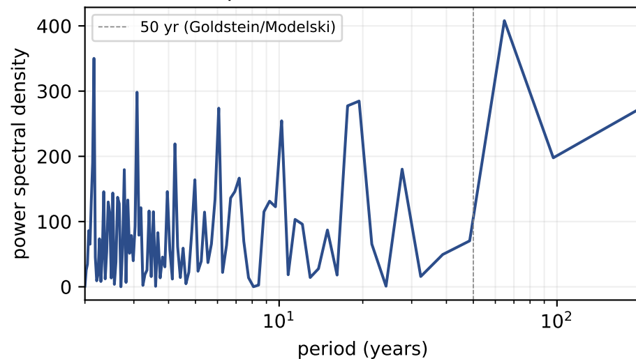
(b) Power spectrum of COW annual war onsets
