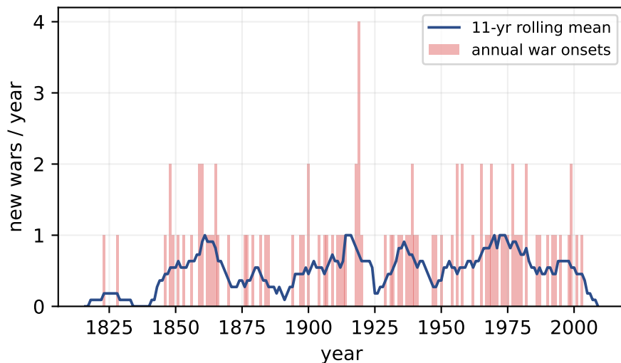
(a) COW war-onset rate 1816-2007
