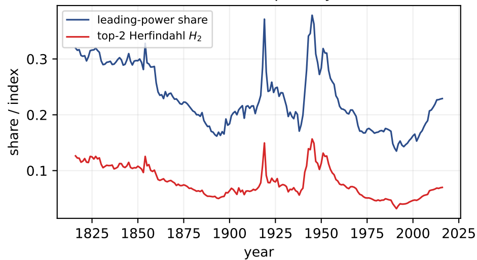
(c) Concentration of capability (NMC v6.0)
