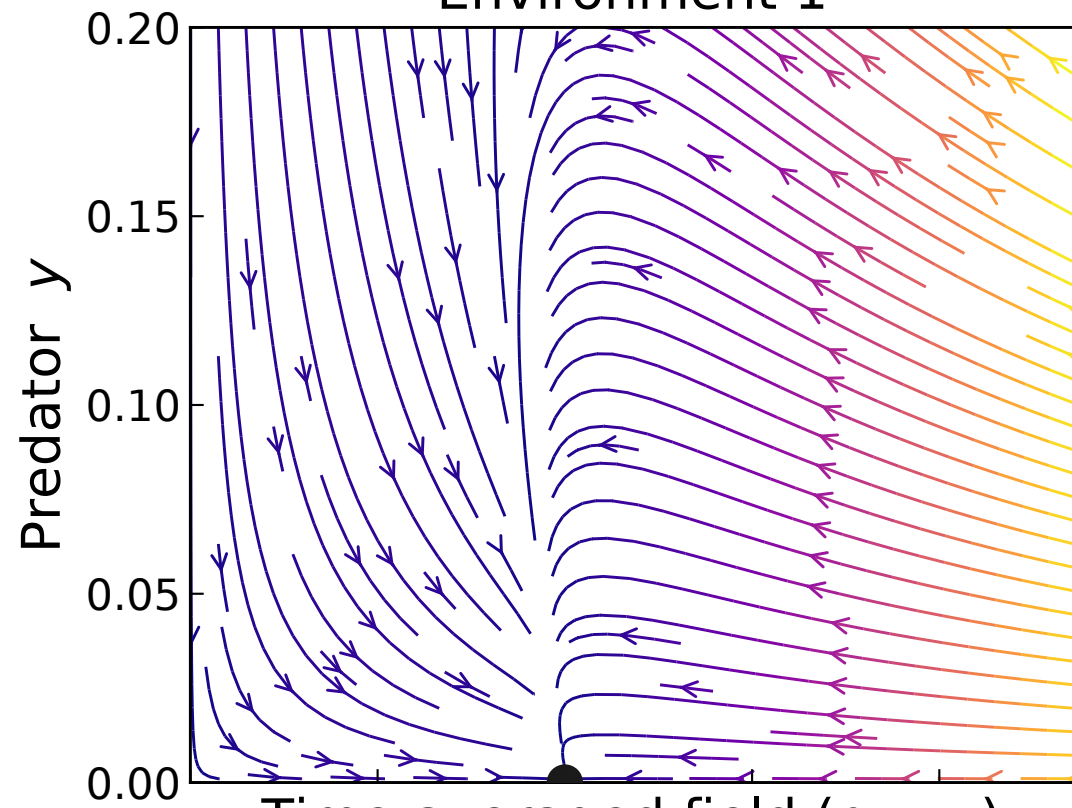
Time-averaged field ( \alpha \rightarrow \infty )
