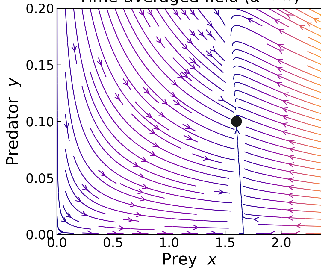
Time-averaged field ( \alpha \rightarrow \infty )
