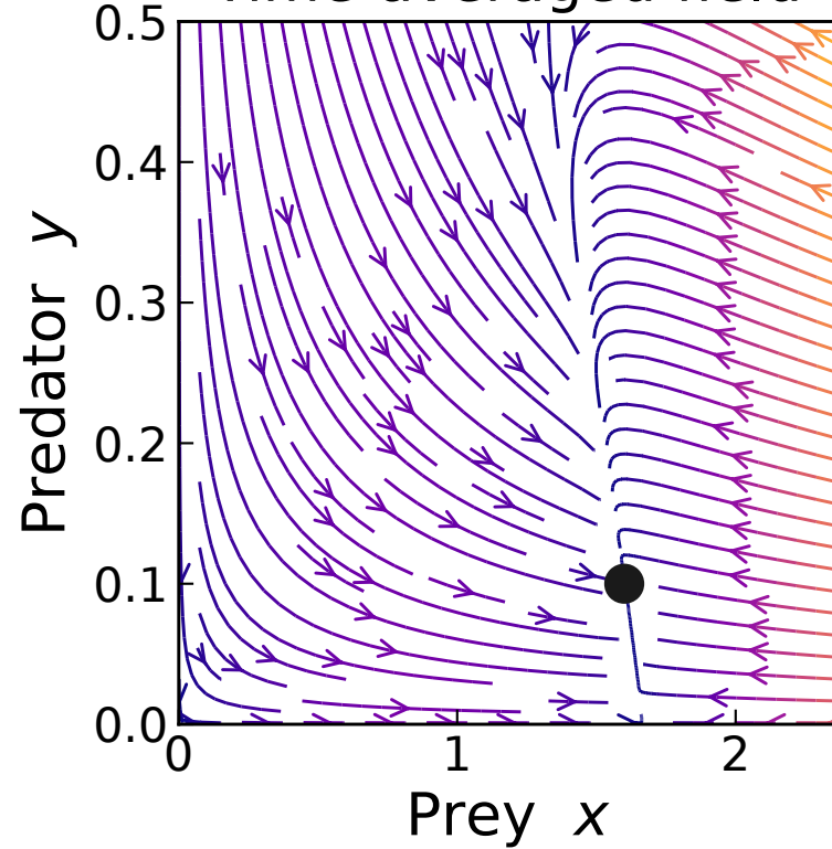
Time-averaged field
