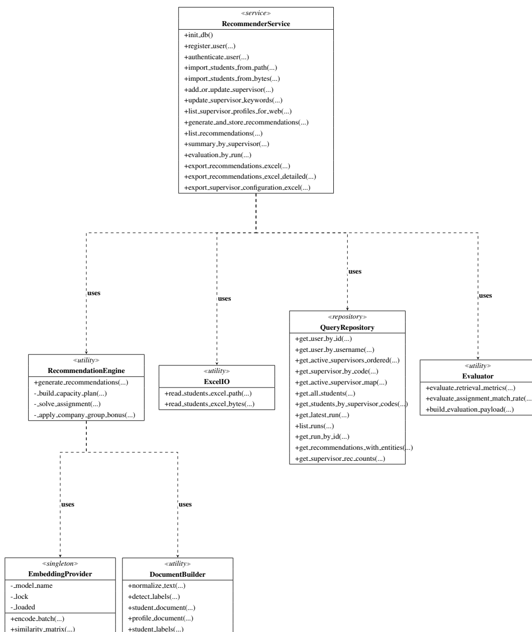
Gambar 3.13. Class Diagram: Service Architecture
