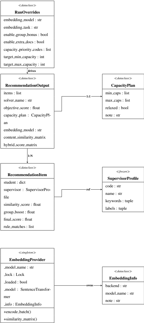
Gambar 3.4. Class Diagram: Runtime Dataclasses
