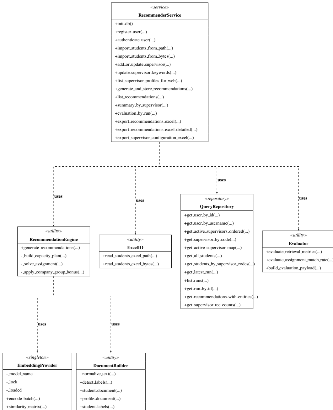
Gambar 3.5. Class Diagram: Service Architecture
