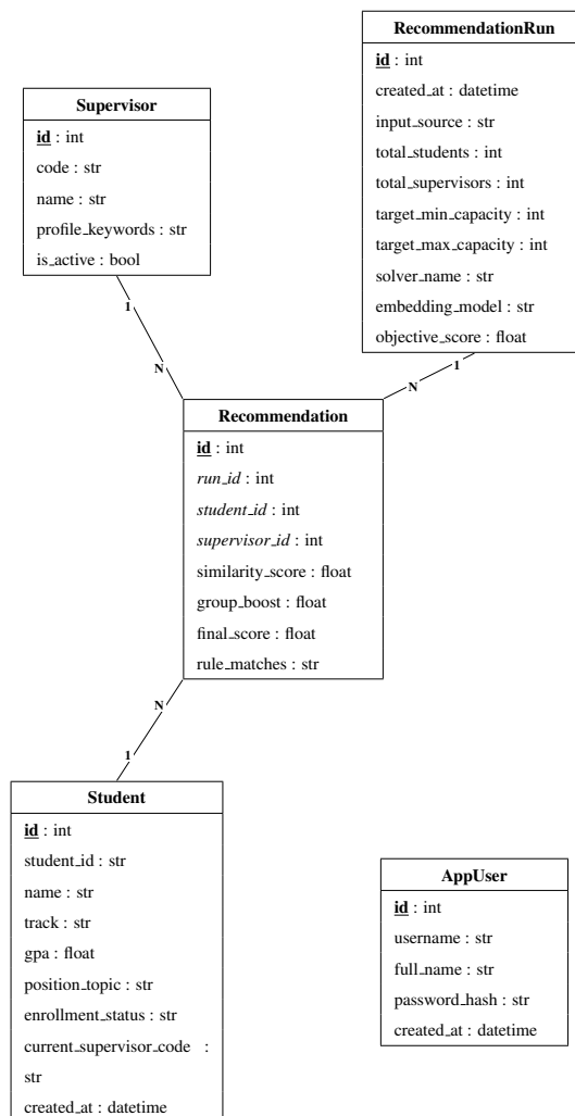
Gambar 3.3. Class Diagram: ORM Models ( id = PK, italic = FK)
