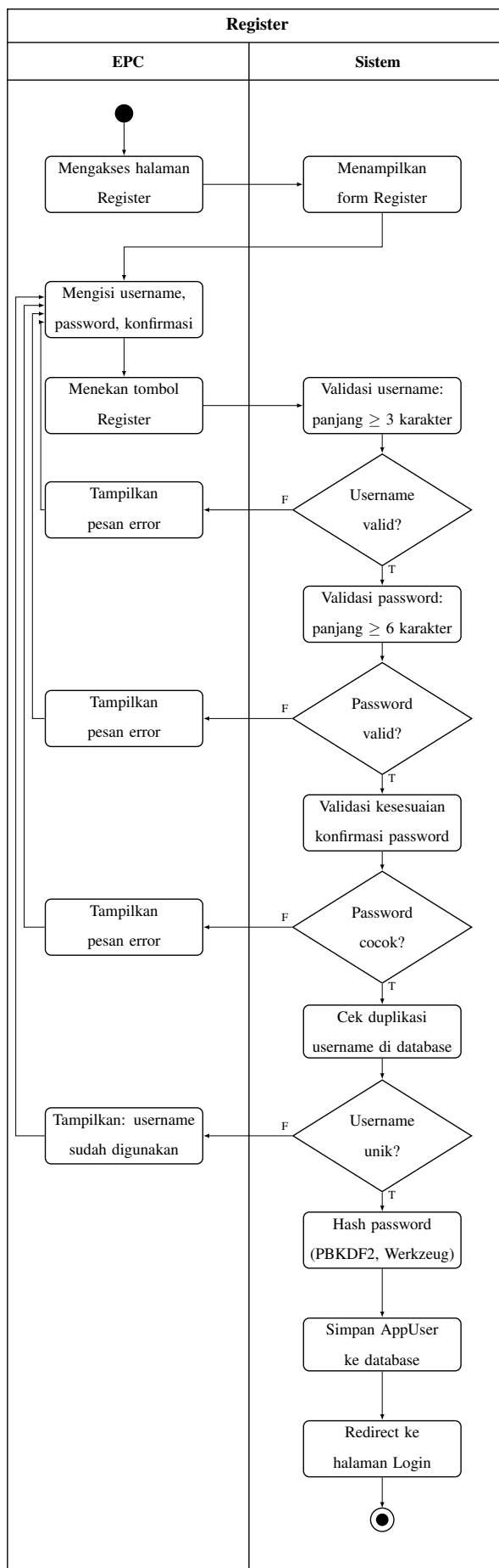
Gambar 3.4. Activity Diagram Register
