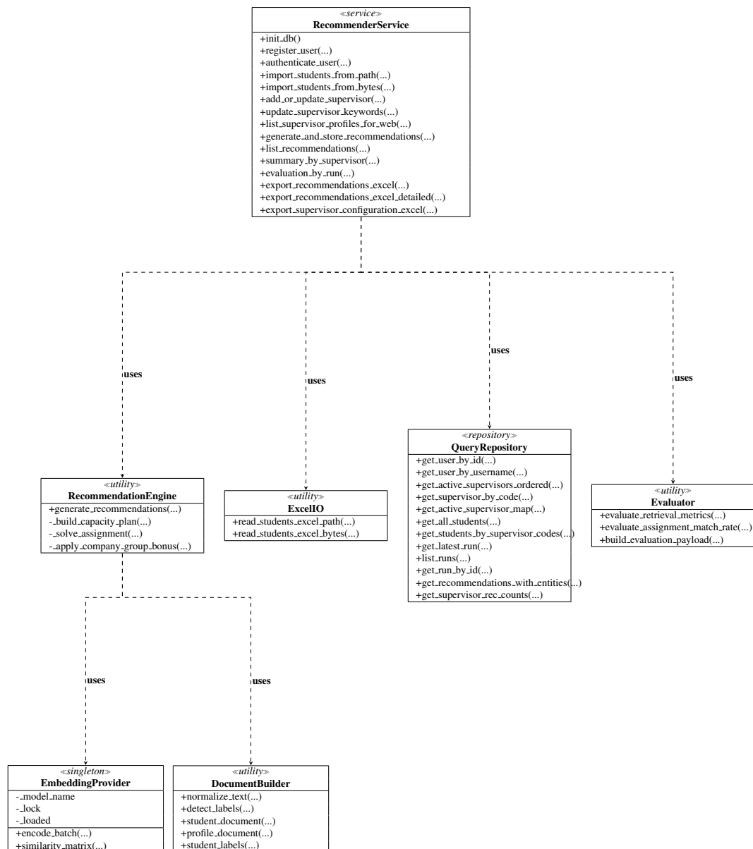
Gambar 3.13. Class Diagram: Service Architecture
